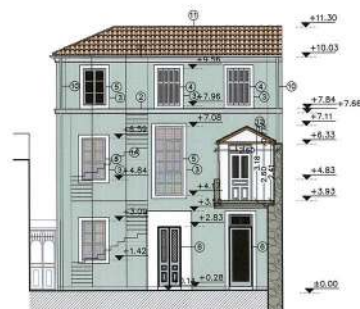
ΟΨΟΤΟΜΗ Α-Α'
