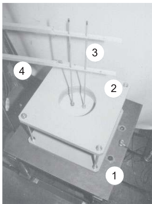
Figure 1.2.2 - Test apparatus
