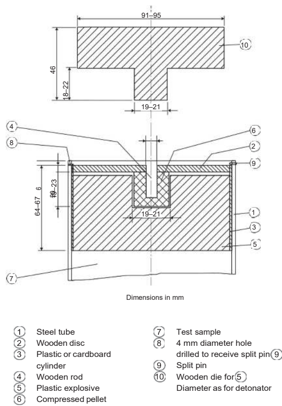
Figure 5-1 - Booster charge
