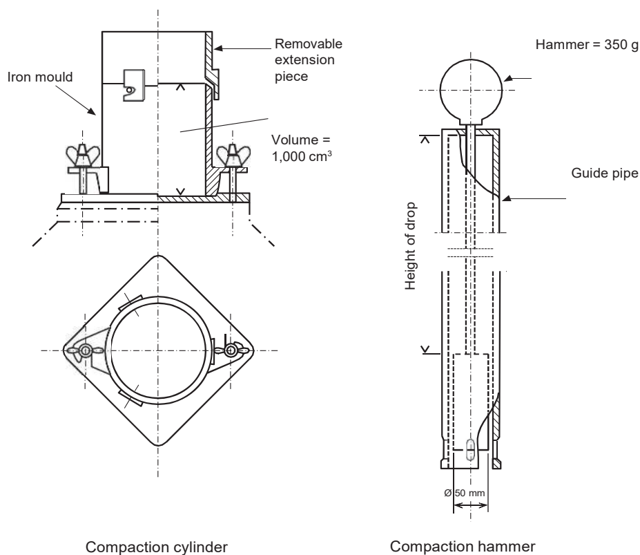
Figure 1.3.2 - Proctor apparatus
